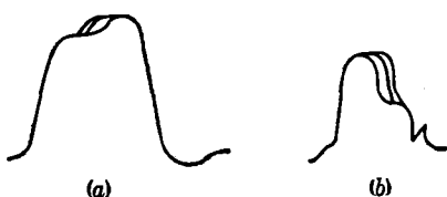
FIG. 8.10.—The pulses of (a) voltage and (b) current that are associated with a mode shift.
